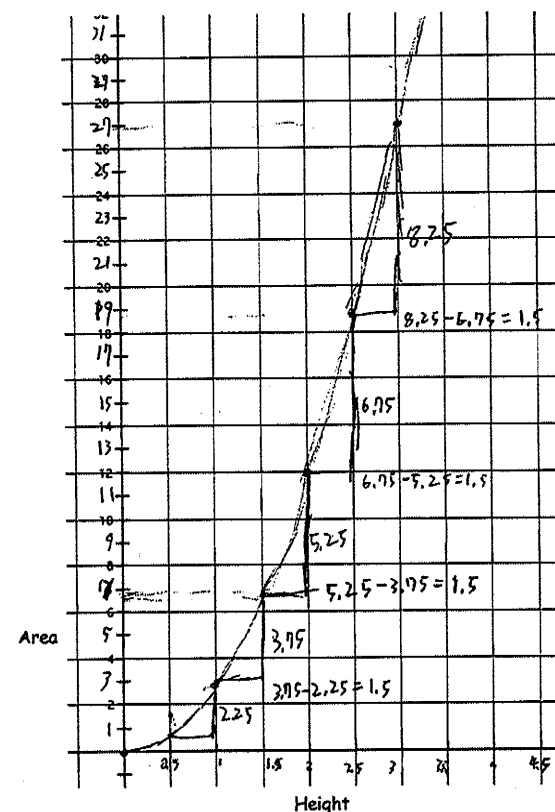
Fig. 16 Daeshim's graph of A = 3h^2
